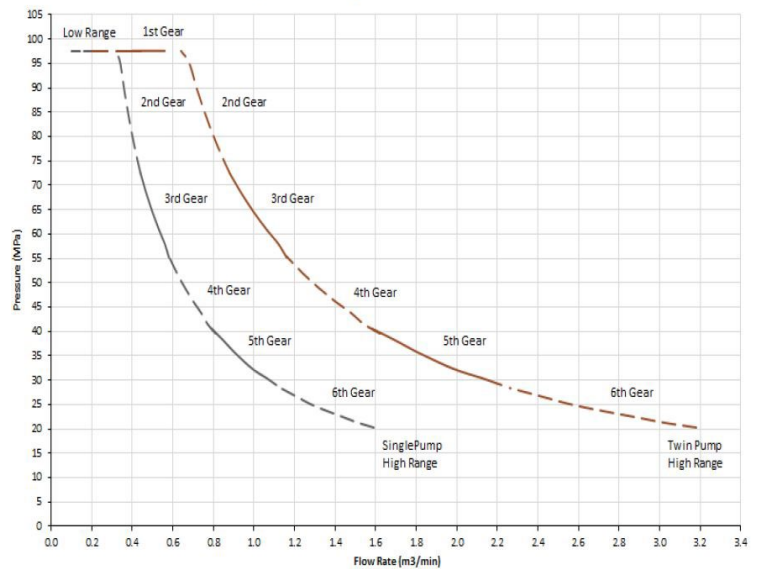
QPA 1000 Pump Performance Chart
